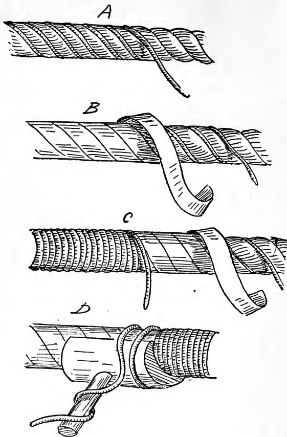
FIG. 138.—Worming, parcelling, and serving.
